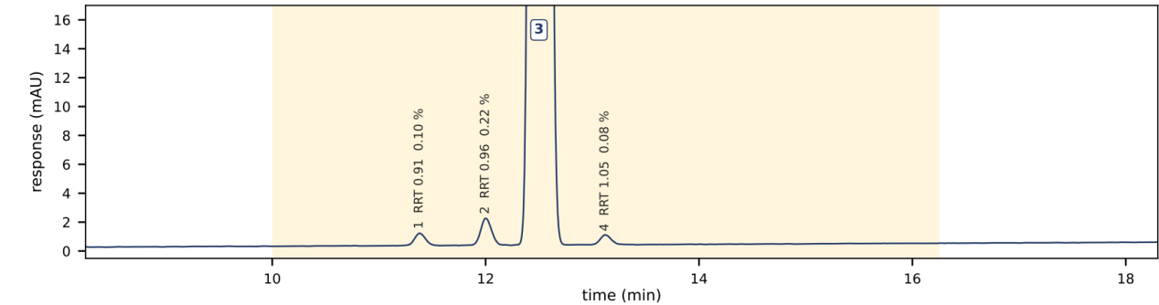
B. Expanded view 0 to 2 % of the main peak height (17.0 mAU); main peak BPC-157 tR 12.50 min off scale; impurities above the 0.05 % reporting threshold, numbered as in the table; yellow band = RRT window 0.80 to 1.30
