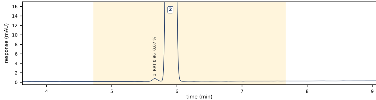
B. Expanded view 0 to 2 % of the main peak height (17.0 mAU); main peak Epithalon tR 5.90 min off scale; impurities above the 0.05 % reporting threshold, numbered as in the table; yellow band = RRT window 0.80 to 1.30
