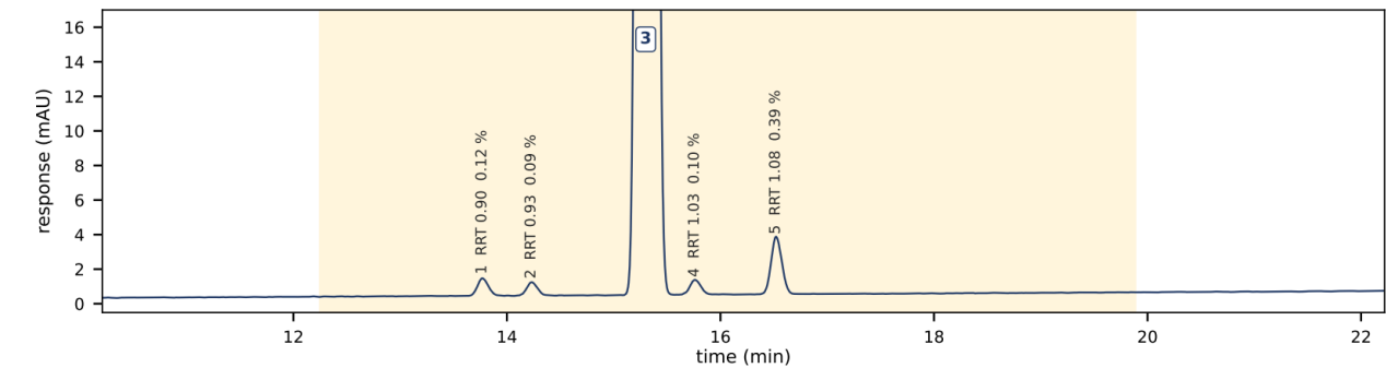
B. Expanded view 0 to 2 % of the main peak height (17.0 mAU); main peak PT-141 tR 15.30 min off scale; impurities above the 0.05 % reporting threshold, numbered as in the table; yellow band = RRT window 0.80 to 1.30
