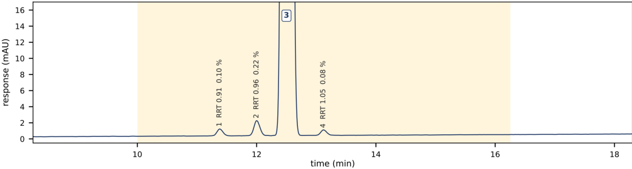
B. Expanded view 0 to 2 % of the main peak height (17.0 mAU); main peak BPC-157 tR 12.50 min off scale; impurities above the 0.05 % reporting threshold, numbered as in the table; yellow band = RRT window 0.80 to 1.30
