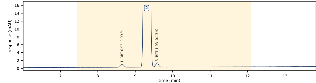
B. Expanded view 0 to 2 % of the main peak height (17.0 mAU); main peak TB-500 tR 9.30 min off scale; impurities above the 0.05 % reporting threshold, numbered as in the table; yellow band = RRT window 0.80 to 1.30
